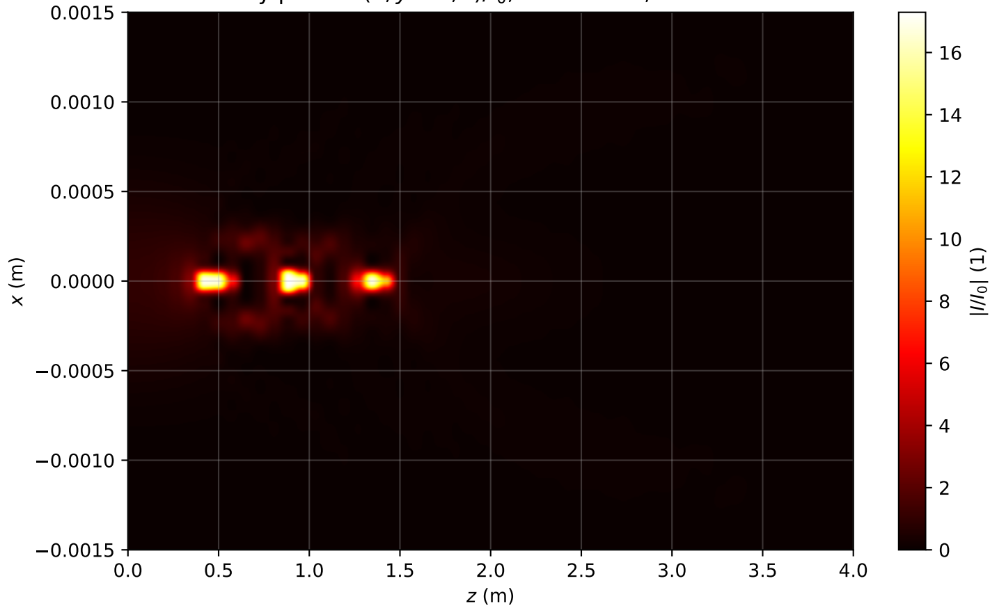
Intensity profile I(x, y = 0, z)/I_0 , P_{in}=6.5P_{cr} , artificial time
